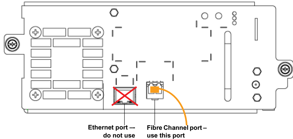
Figure 3 IBM LTO-5 and LTO-6 Single Port Fibre Channel Tape Drive
