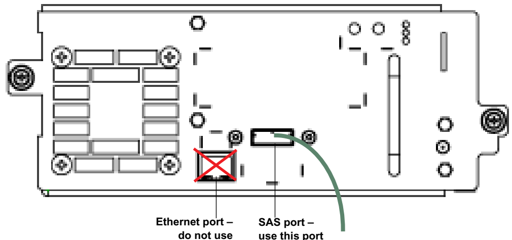
Figure 2 HP LTO-5 and LTO-6 Single Port SAS Tape Drive
