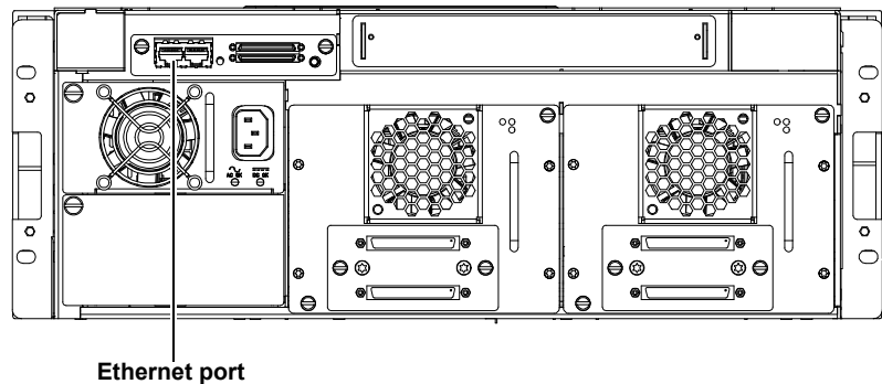
Figure 129 Connecting to the Library SCB
