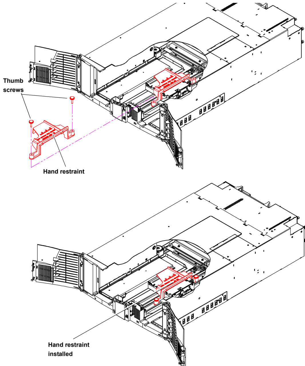
Figure 124 Installing the Hand Restraint
