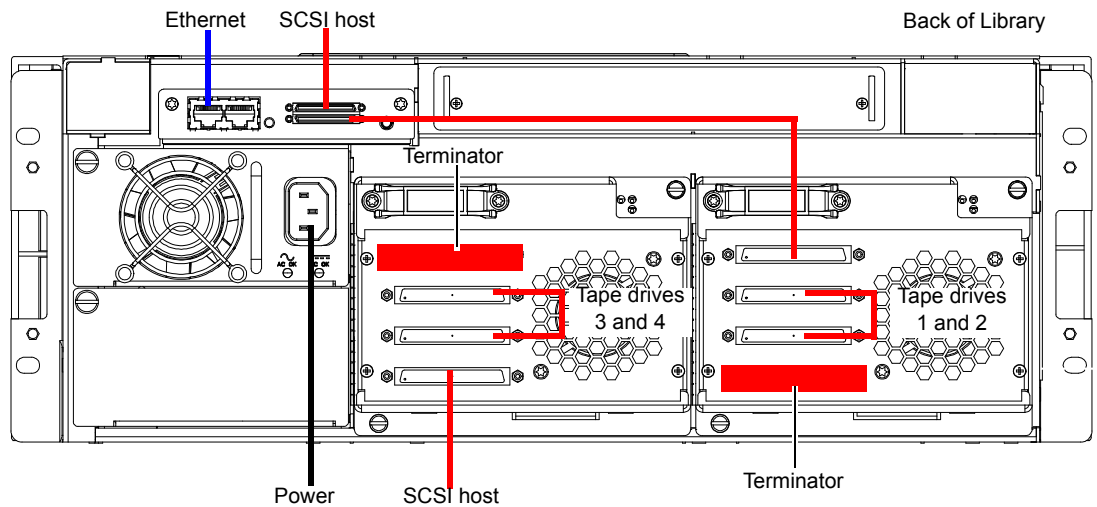
Figure 112 Scalar 50 Cable Configuration (SCSI Half-Height Drives)
