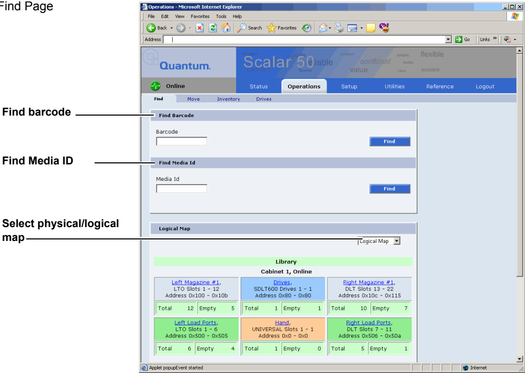
Figure 53 Find Page
