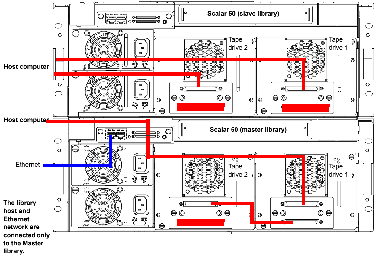
Figure 114 Scalar 50 Cable Configuration (Stacked)
