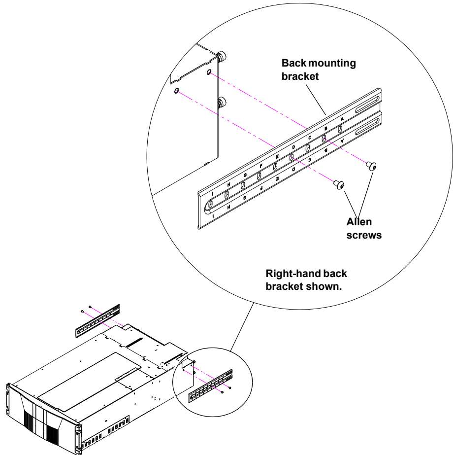
Figure 106 Back Mounting Brackets
