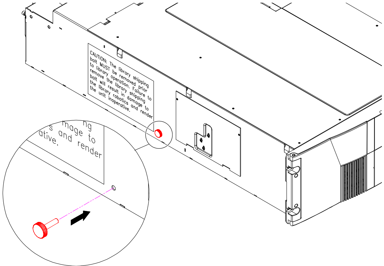
Figure 125 Installing the Restraining Bolt
