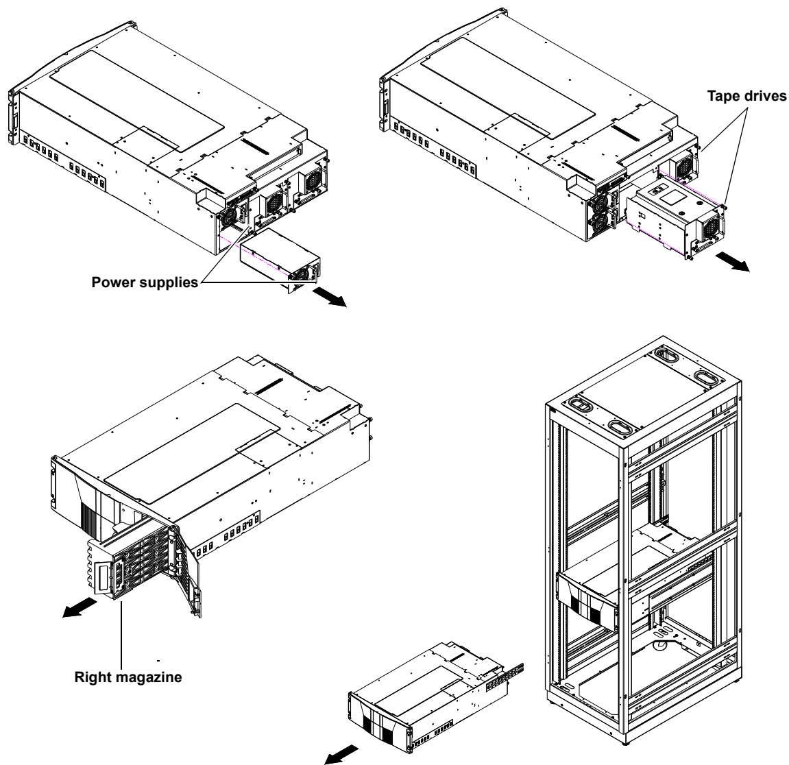
Figure 122 Removing the Scalar 50 Library
