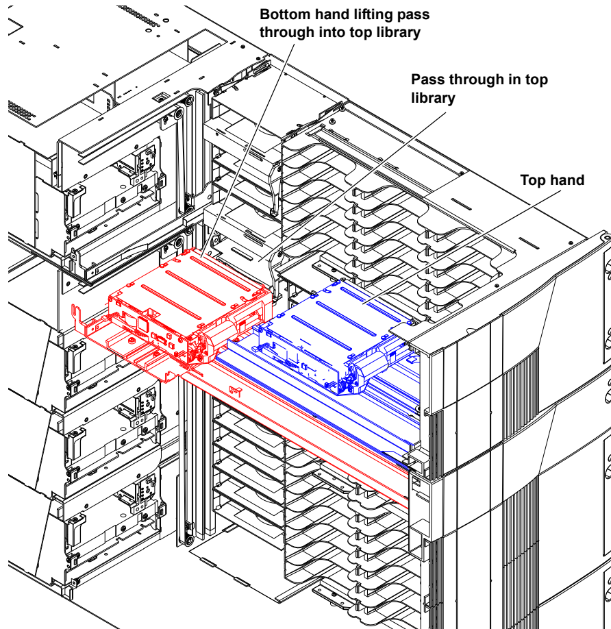
Figure 7 Multiple Library Stack (Cross Section
