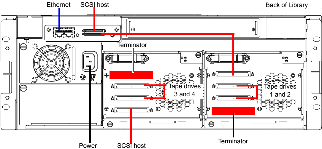
Figure 18 Scalar 50 Cable Configuration (SCSI Half-Height Drives)
