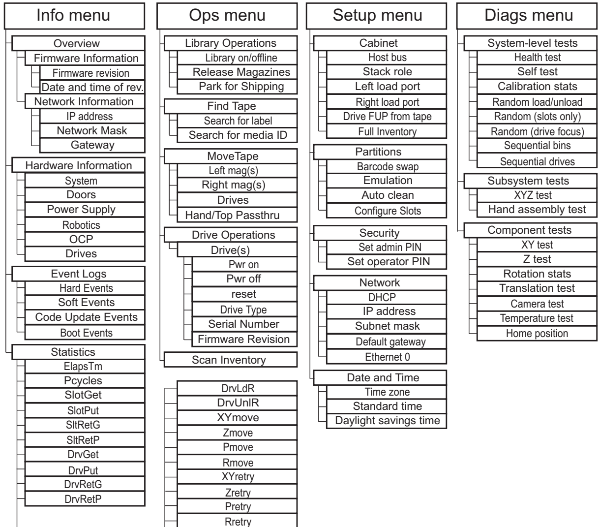
Figure 23 OCP Component Tree
