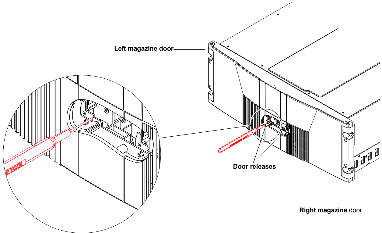
Figure 120 Opening the Right and Left Magazine Access Doors
