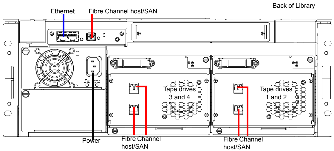
Figure 113 Scalar 50 Cable Configuration (Native Fibre Channel Half-Height Drives)
