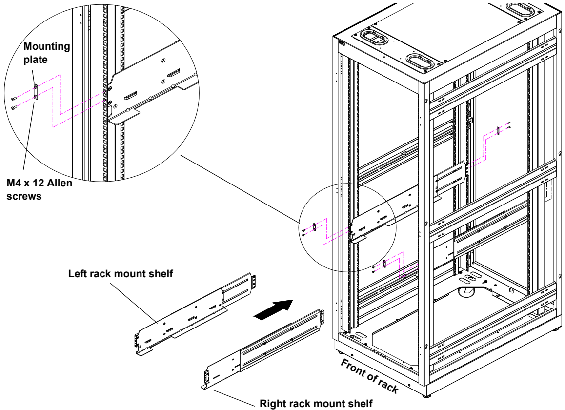
Figure 105 Installing the Rack Mount Shelves
