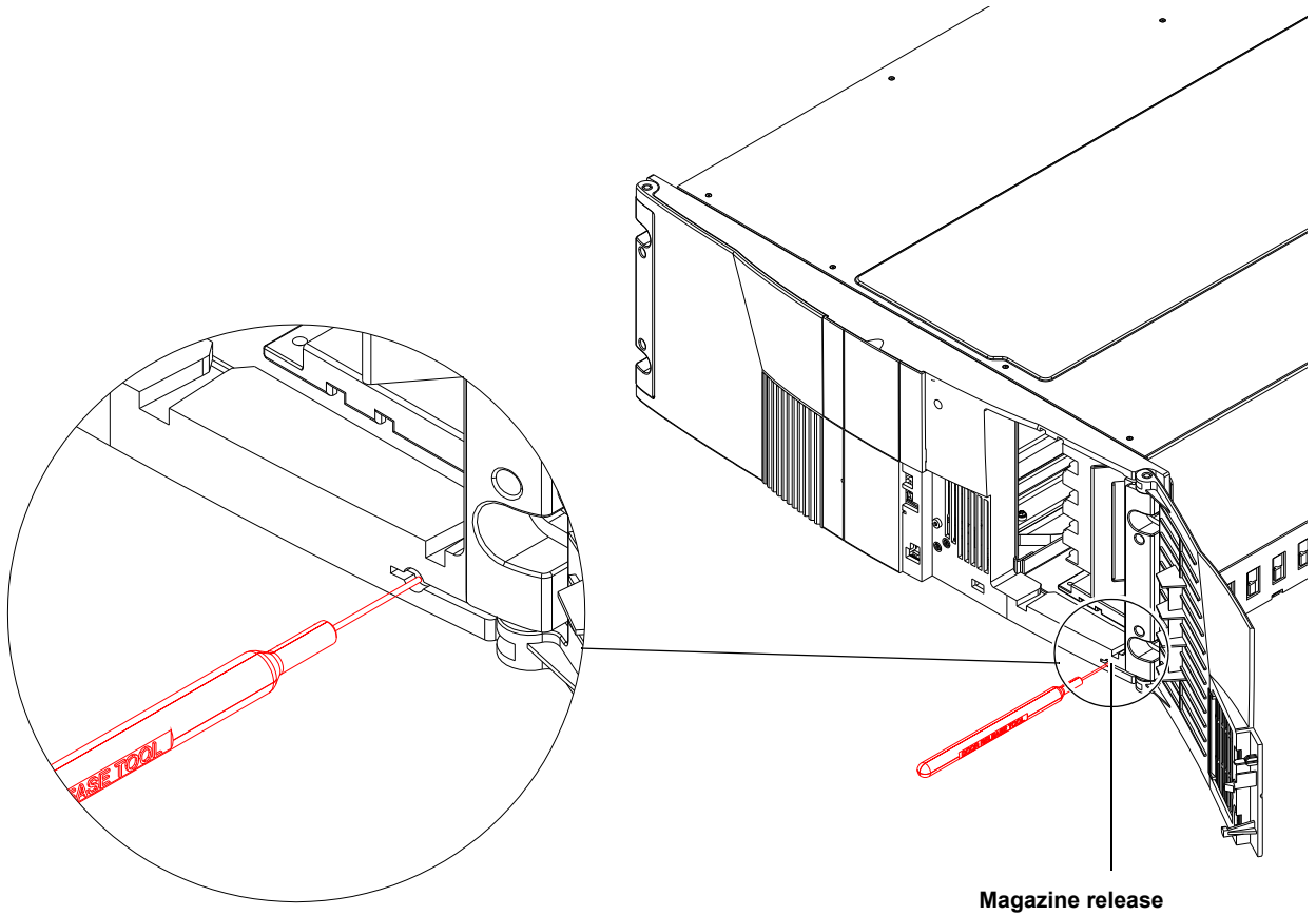
Figure 121 Removing the Magazines
