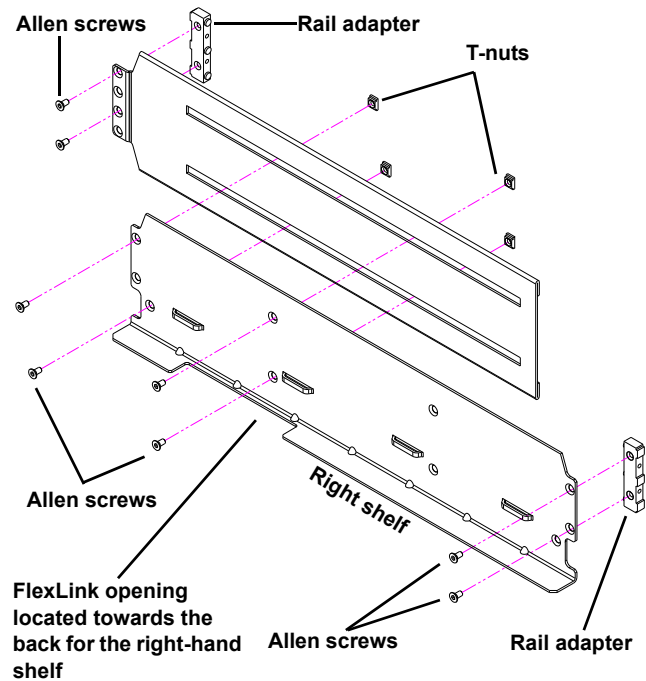
Figure 104 Assembling the Right-Hand Rack Mount Shelves
