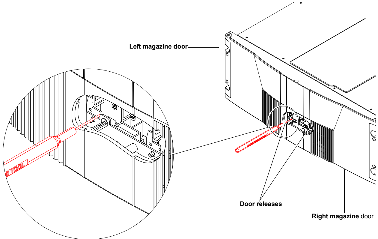
Figure 123 Opening the Right and Left Magazine Access Doors
