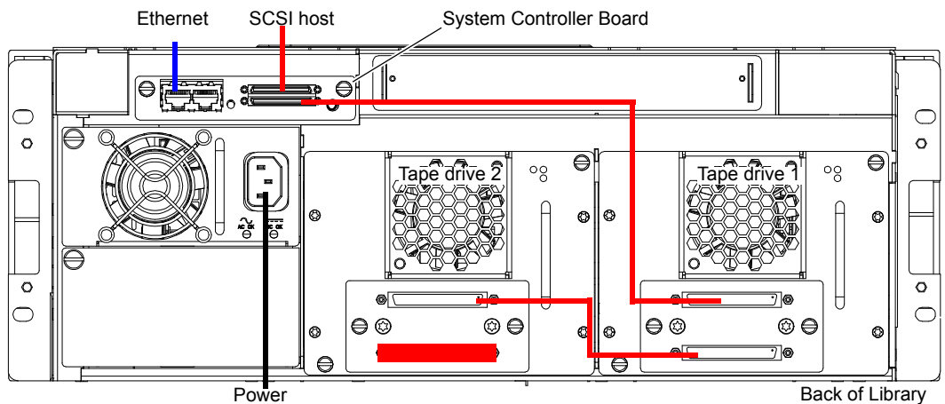
Figure 110 Scalar 50 Cable Configuration (SCSI Full Height Drives)
