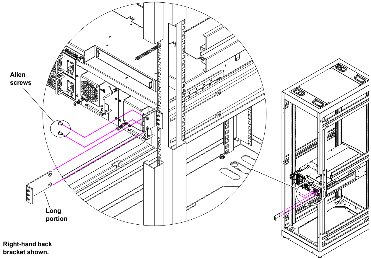
Figure 108 Securing the Back of the Library
