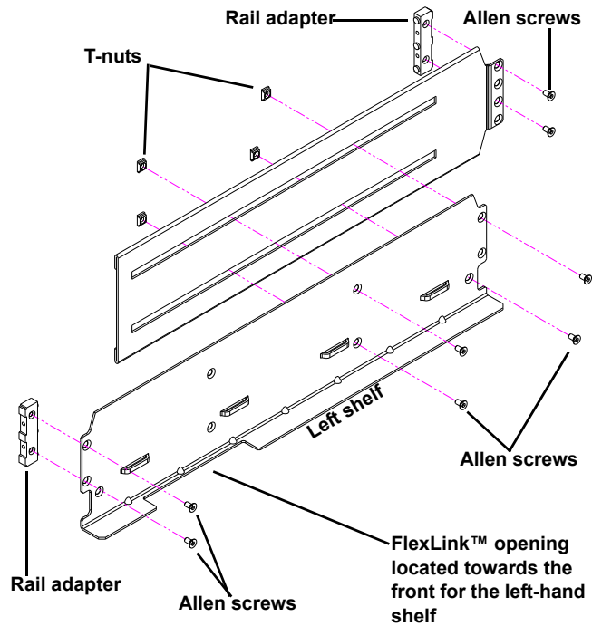
Figure 103 Assembling the Left-Hand Rack Mount Shelves
