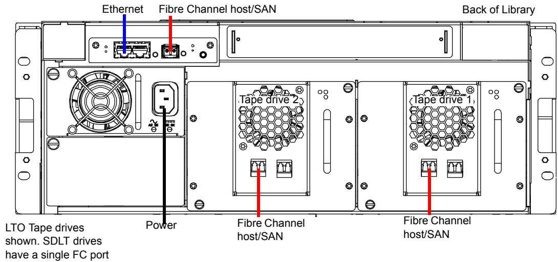
Figure 111 Scalar 50 Cable Configuration (Native Fibre Channel Full Height Drives)
