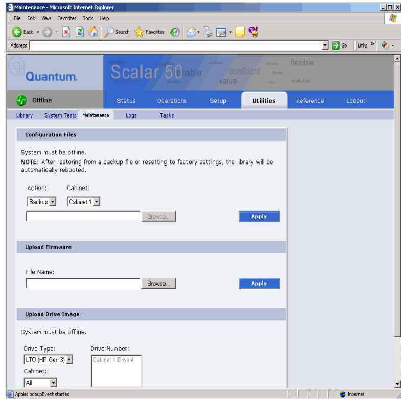
Figure 132 Maintenance Page
