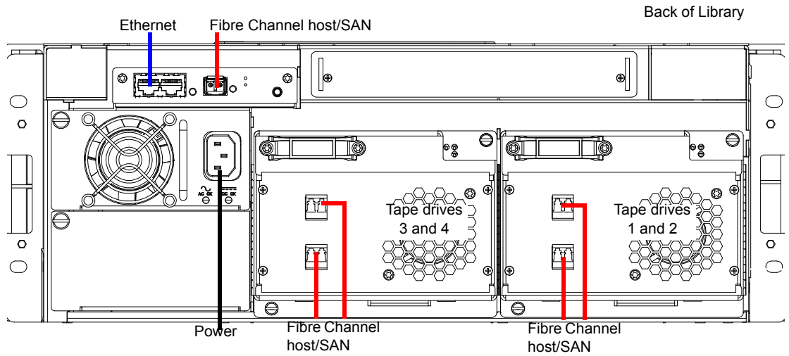
Figure 19 Scalar 50 Cable Configuration (Native Fibre Channel Half-Height Drives)
