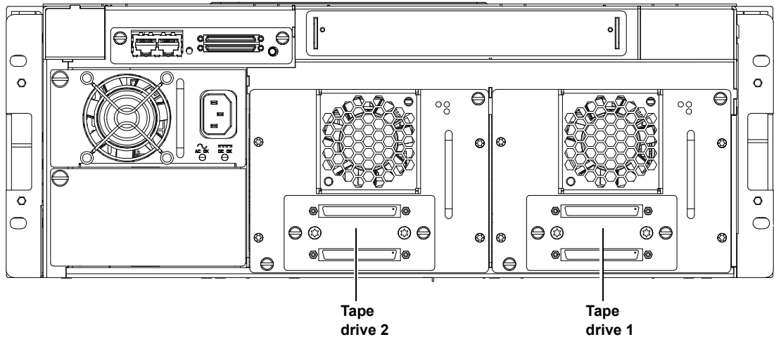
Figure 109 Scalar 50 Tape Drive Numbering
