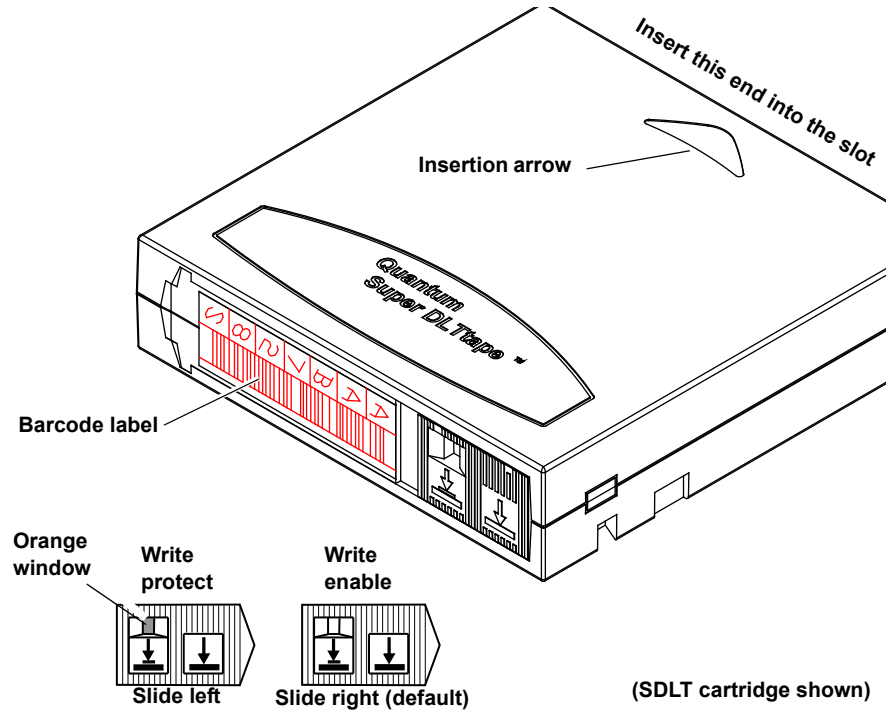
Figure 11 SDLT Cartridges
